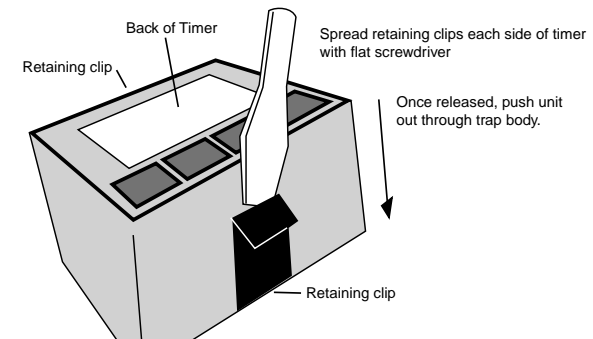
FIG. 9.3 – Removal of Timer Unit
