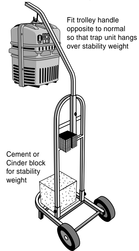
FIG. 2.4 Trolley assembly option
