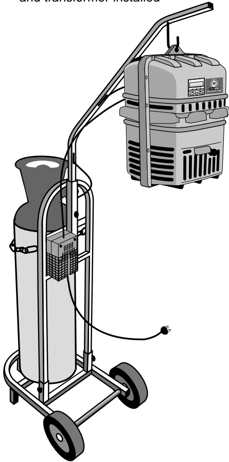
FIG. 2.2 Trolley assembly
