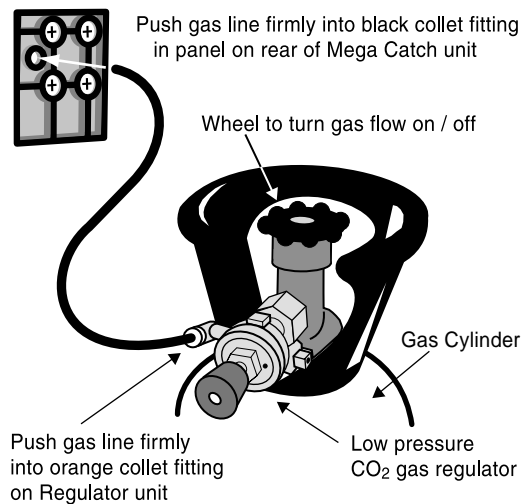
FIG. 3.2 Connection of Trap to CO 2 gas cylinder
